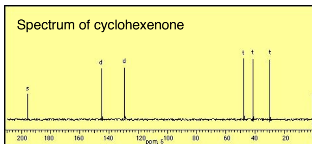
Cyclohexenone
