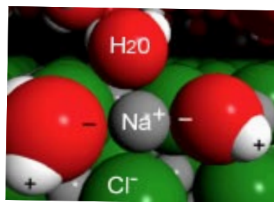
VisChem animation from depicting the hydration of a \text{Na}^+ ion on a NaCl surface.
